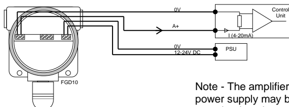
Figure 4 – Analogue Output
